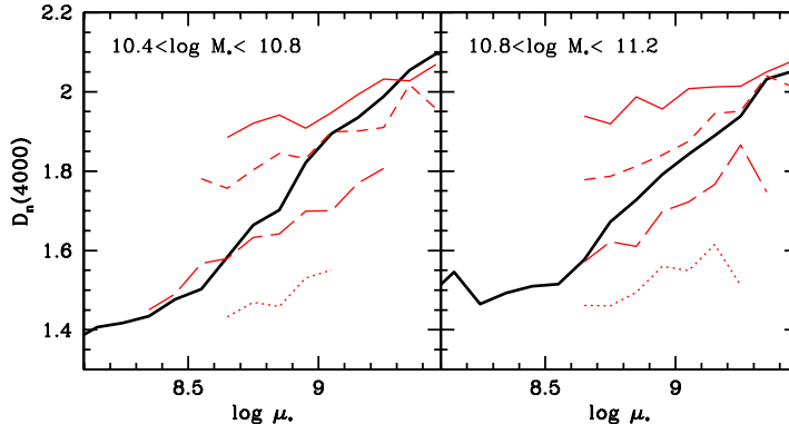
Figure 15: The thick black lines show the median relation between D_n(4000) and \log \mu_* for normal galaxies in two different ranges in stellar mass. The red lines show the median relation for the host galaxies of AGN with \log L[\text{OIII}] < 6.0 (solid), 6.0 < \log L[\text{OIII}] < 7.0 (short-dashed), 7.0 < \log L[\text{OIII}] < 8.0 (long-dashed) and \log L[\text{OIII}] > 8.0 (dotted).
